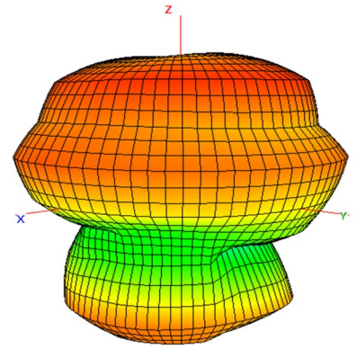
5850 MHz
