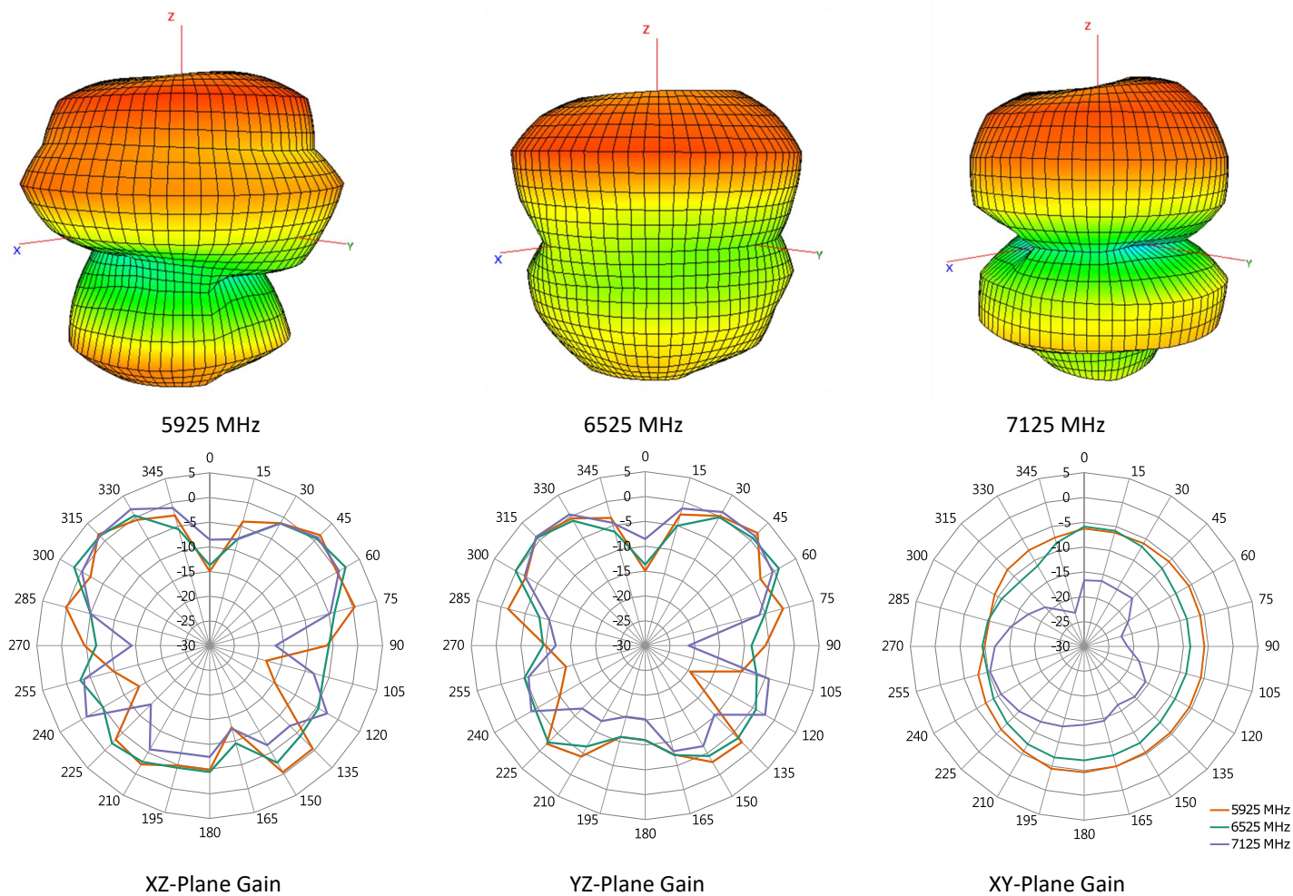
Figure 9-1. Antenna Radiation Patterns, Bent 90 Degrees
