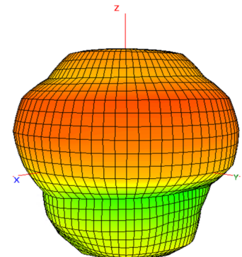
5000 MHz
