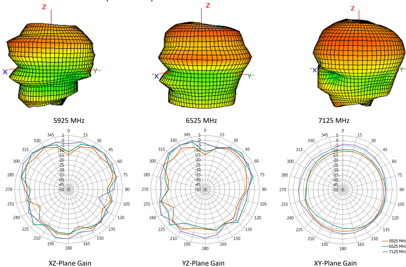
Figure 9-1. Antenna Radiation Patterns, Straight without ground plane
