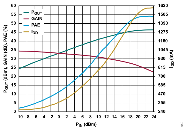
Figure 42. P_{OUT} , Gain, PAE, and I_{DD} vs. P_{IN} at 3.1 GHz
