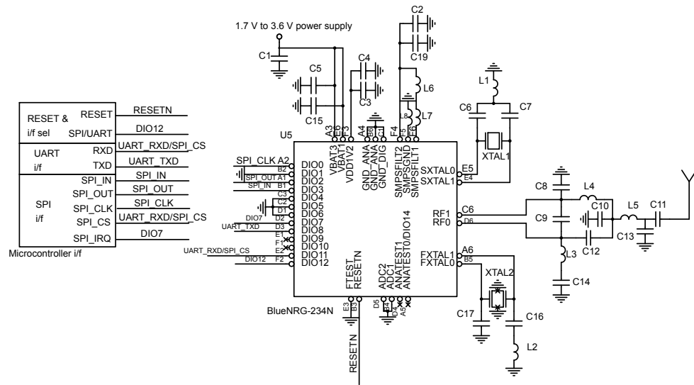
Figure 11. Application circuit: active DC-DC converter WLCSP34 package
