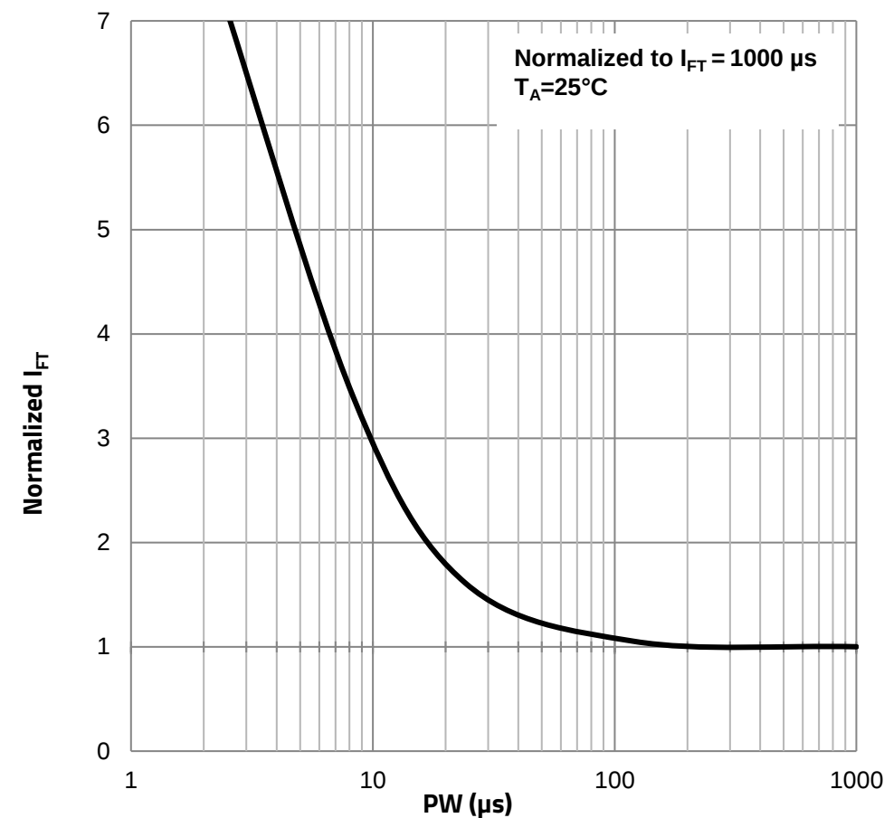
Normalized Trigger Current vs. LED Trigger Pulse Width:
