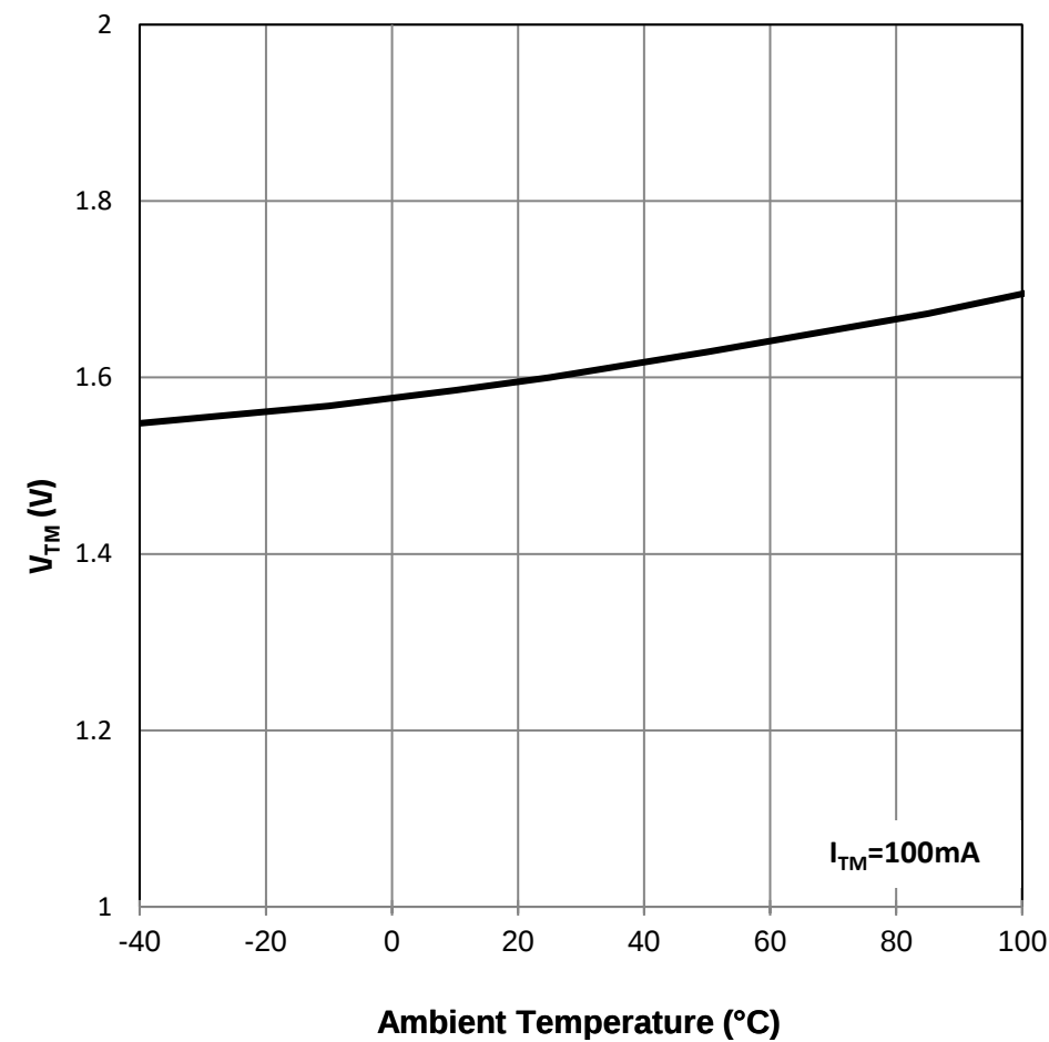
Peak On-State Terminal Voltage vs. Ambient Temperature:
