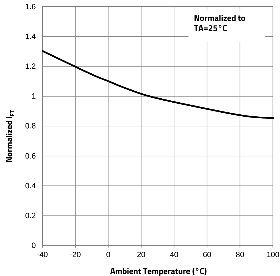
Normalized Trigger Current vs. Ambient Temperature:
