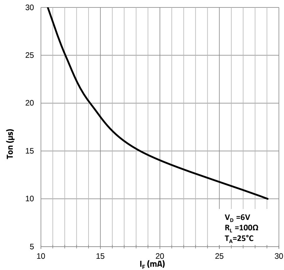
Turn on Time vs. Forward Current:
