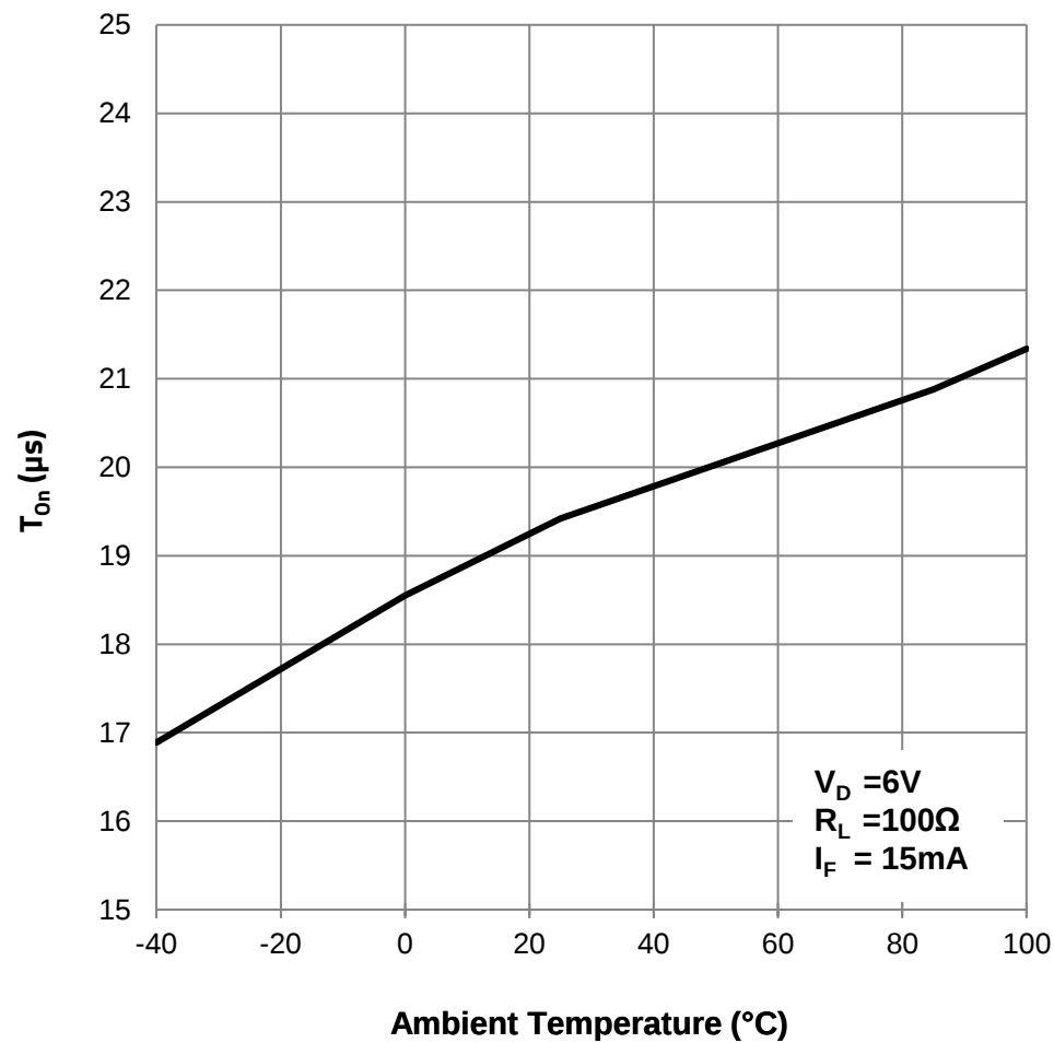
Turn On Time vs. Ambient Temperature:
