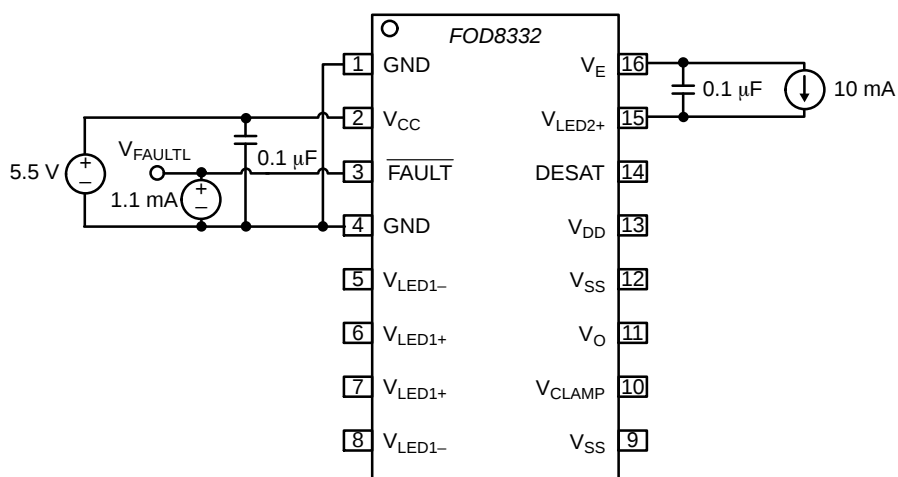
Figure 46. FAULT Low Level Output Voltage ( V_{FAULTL} ) Test Circuit
