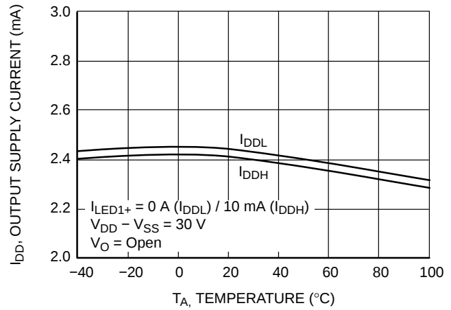
Figure 12. Output Supply Current ( I_{DD} ) vs. Temperature
