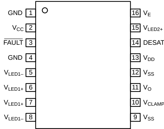
Figure 1. Pin Configuration
