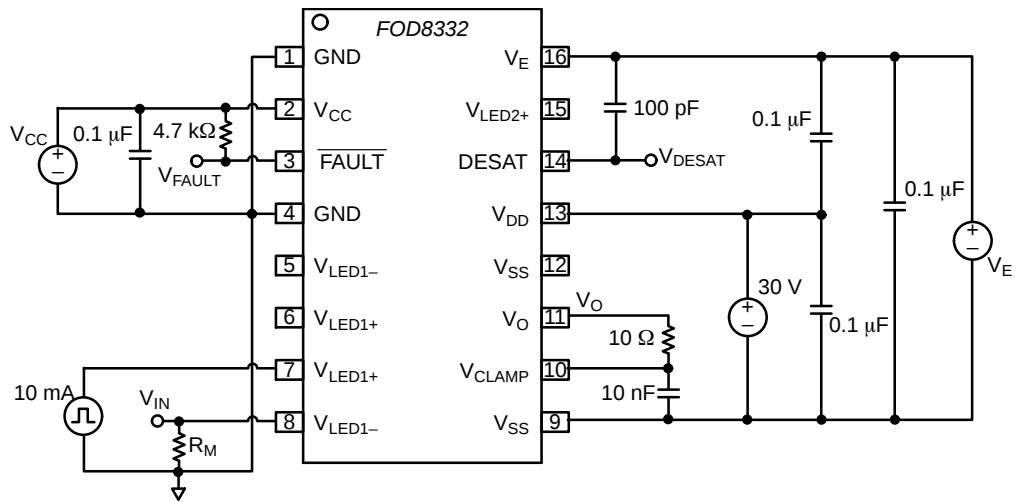
Figure 48. DESAT Sense Delay ( t_{\text{DESAT}(90\%)} ), t_{\text{DESAT}(10\%)} , t_{\text{DESAT}(\text{LOW})} , DESAT Sense to Low Level FAULT Signal Delay ( t_{\text{DESAT}(\text{FAULT})} ), Reset to High Level FAULT Signal Delay ( t_{\text{RESET}(\text{FAULT})} ), DESAT Input Mute ( t_{\text{DESAT}(\text{MUTE})} ) Test Circuit
