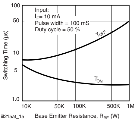
Fig. 15 - Typical Switching Characteristics vs. Base Resistance (Saturated Operation)
