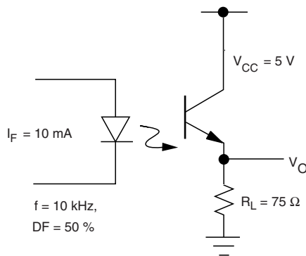
Fig. 2 - Non-Saturated Switching Timing
