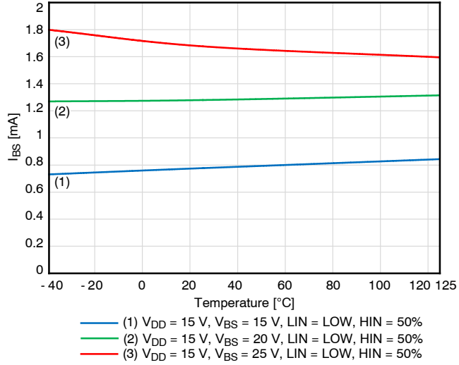
Figure 14. I_{BS} Supply Current V_{BS} = 15\text{--}25\text{ V} , HIN = 20\text{ kHz} / 50\%
