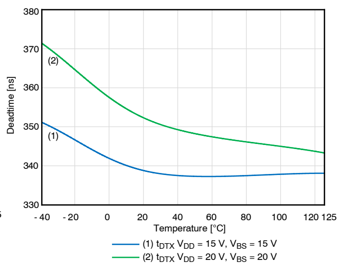
Figure 25. Deadtime
