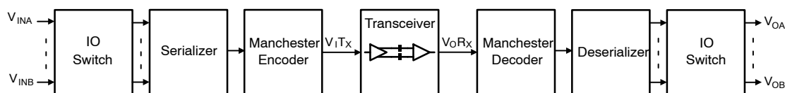
Figure 11. Operational Block Diagram of Multi-Channels
