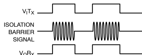
Figure 13. On-Off Keying Modulation Signals
