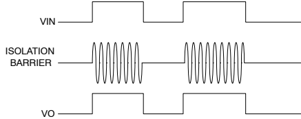
Figure 14. On-Off Keying Modulation Signals
