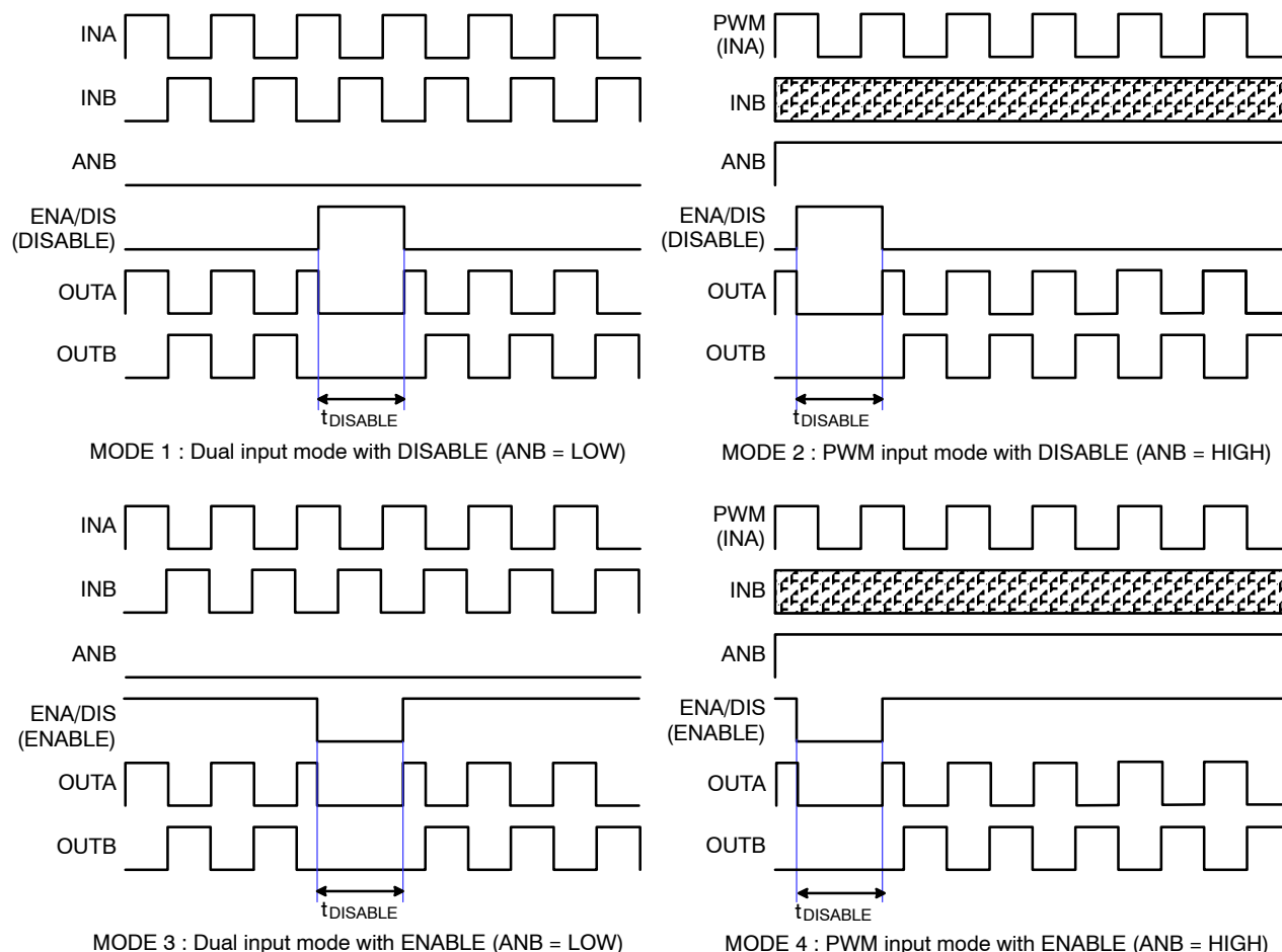
Figure 53. Timing Chart of ENABLE and DISABLE Modes
