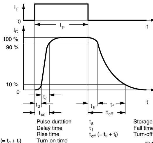
Fig. 3 - Switching Times
