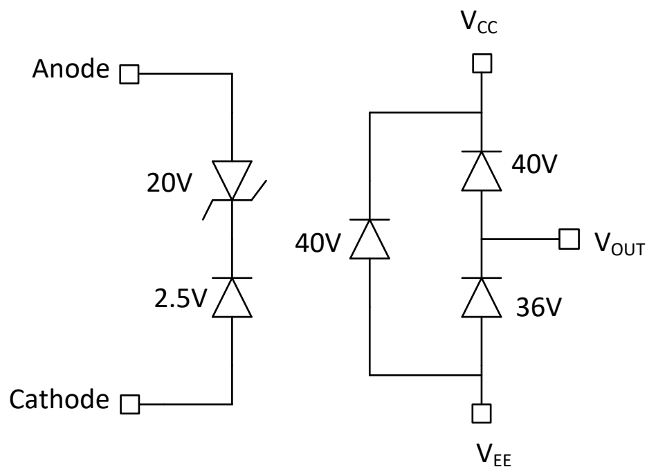
Figure 8-6. ESD Structure
