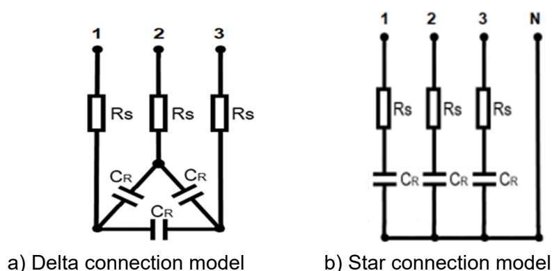
Figure 8: Resistance model of 3 Phase capacitor
