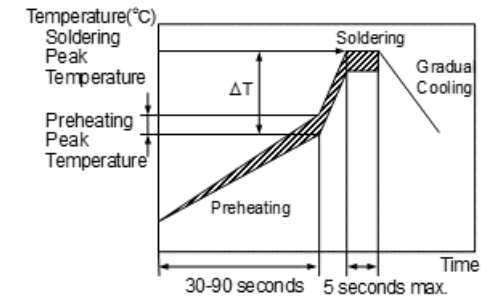
[ Standard Conditions for Flow Soldering ]
