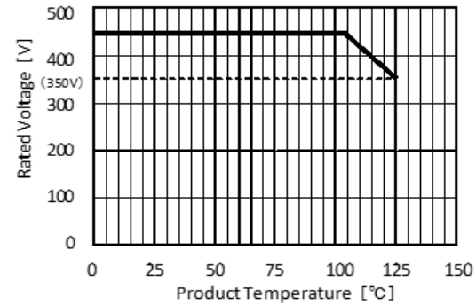
Fig:Derating
