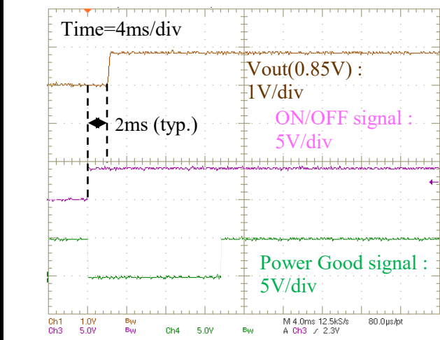
On/Off Enable Delay (Vin=5.0V, Vout=0.85V, Iout=0A, Load=110uF)
