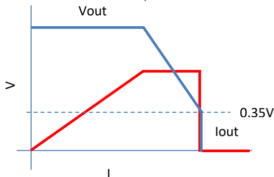
Latch-off short circuit protection
