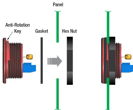
Figure 2. Panel Installation
