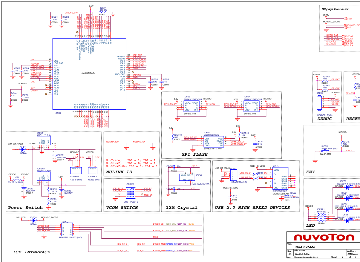
Figure 4.1-1 Nu-Link2-Me Circuit
