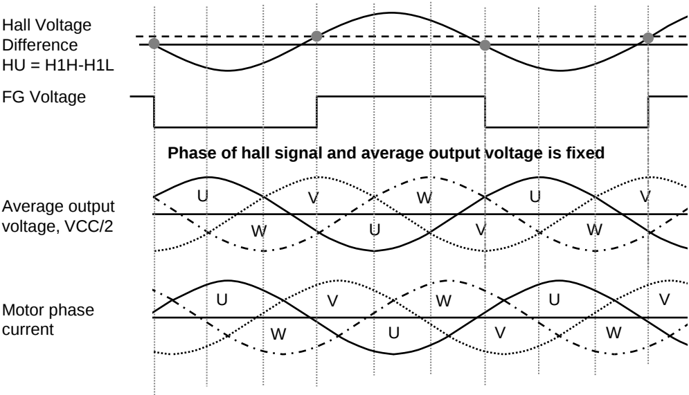
Fixed to 0 deg when PS=High
