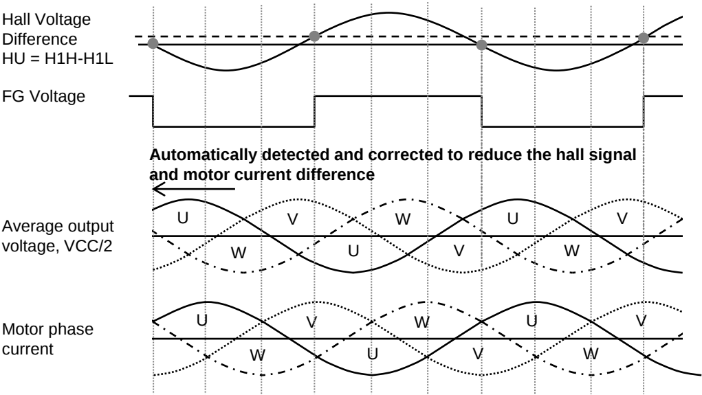
Automatic drive phase shift control when PS=Low
