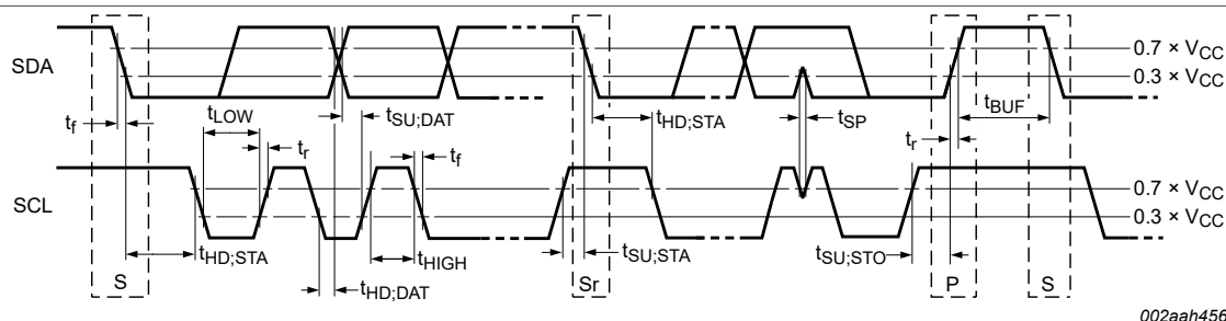
Figure 31. Timing diagram
