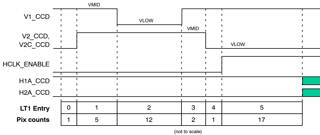
Figure 5. Line Table 1 Default Timing
