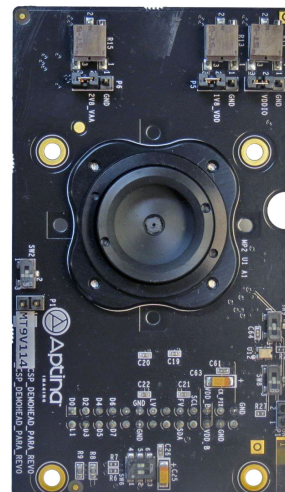
Figure 1. MT9V114 Evaluation Board
