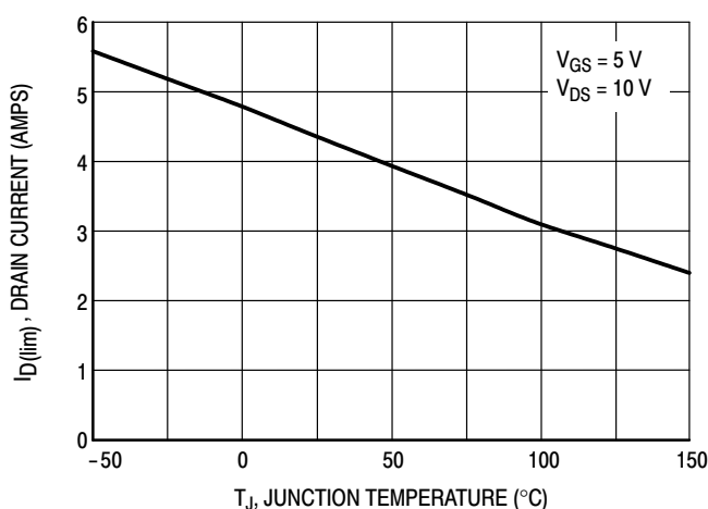
Figure 3. I_{D(Im)} Variation With Temperature
