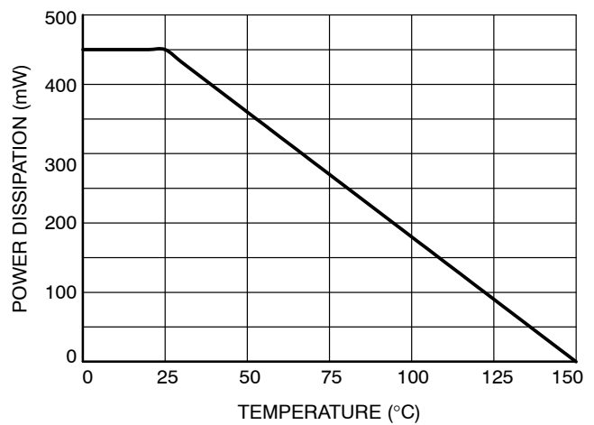
Figure 6. Derating Curve
