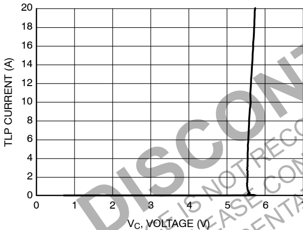
Figure 3. Positive TLP I-V Curve, Pin 2 to Pin 1
