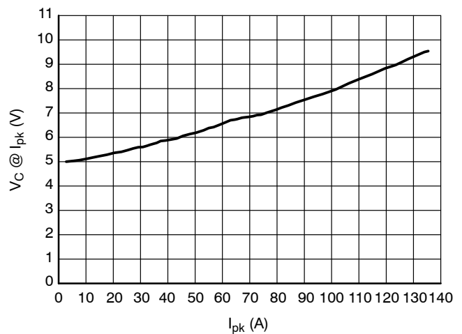
Figure 6. Clamping Voltage vs. Peak Pulse Current ( t_p = 8/20 \mu s ), Pin 1 to Pin 2
