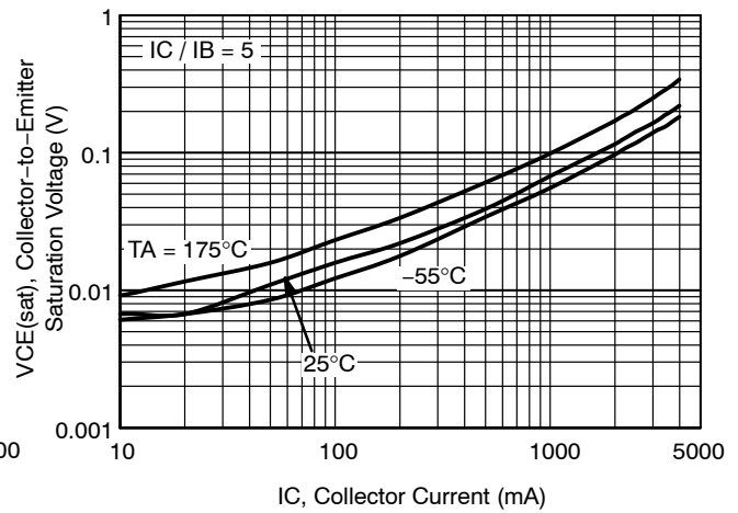
Figure 5. V_{CE(sat)} - I_C
