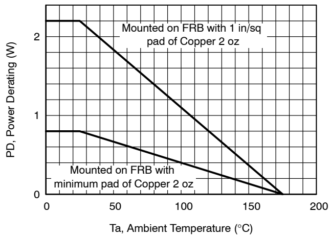
Figure 12. Power Derating
