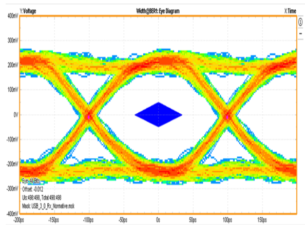
With ESD8016
