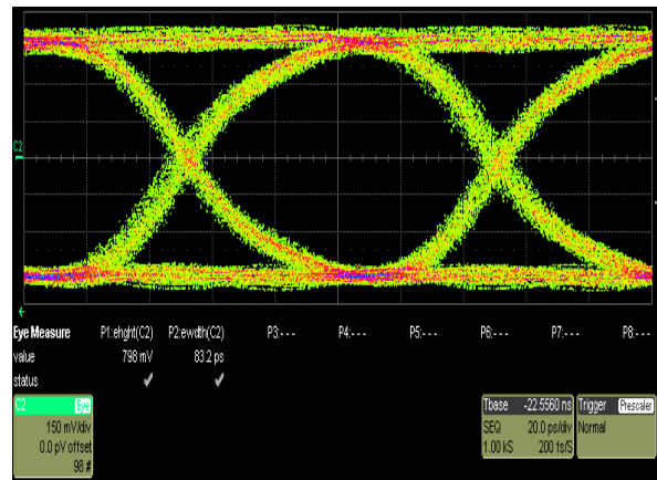
With ESD8016
