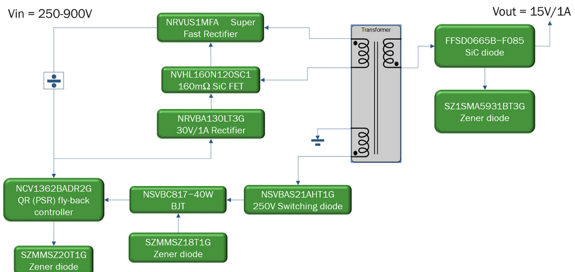
Figure 3. Block Diagram
