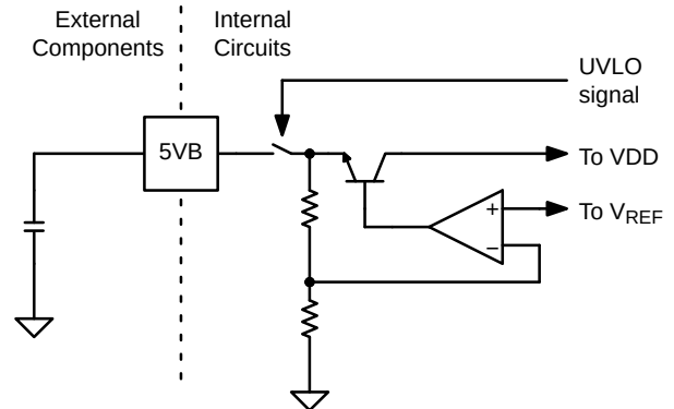
Figure 17. 5 V Bias
