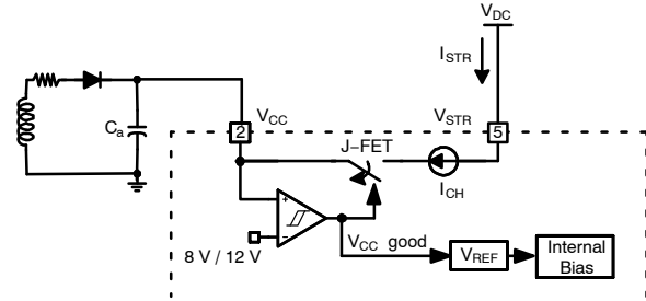
Figure 14. Startup Circuit
