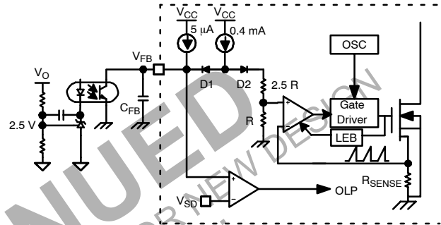
Figure 16. Pulse-Width-Modulation Circuit
