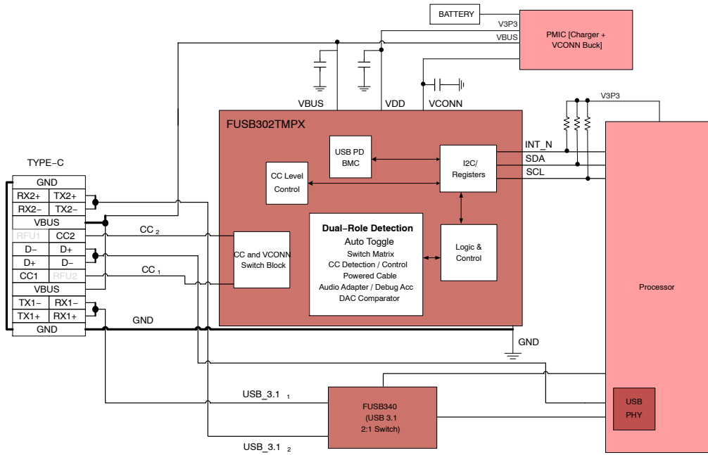
Figure 2. Typical Application
