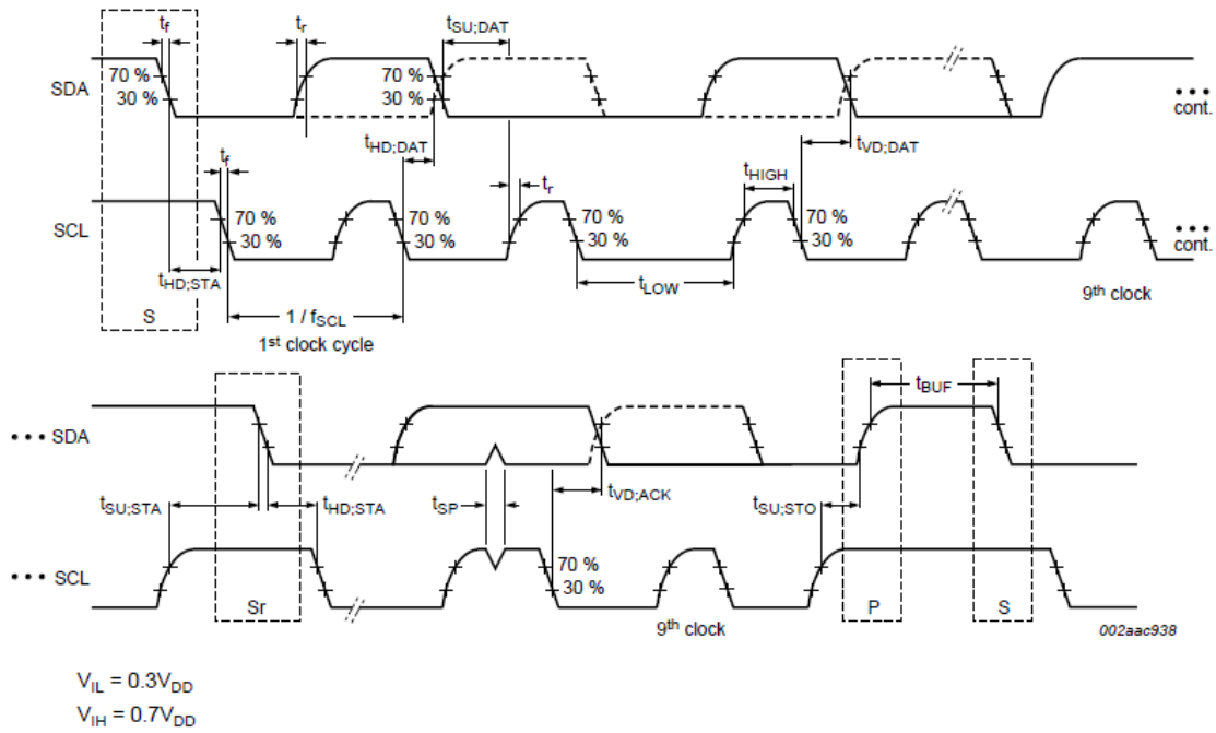
Figure 15. Definition of Timing for Full-Speed Mode Devices on the I²C Bus
