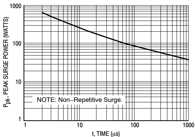
Figure 9. Pulse Width
