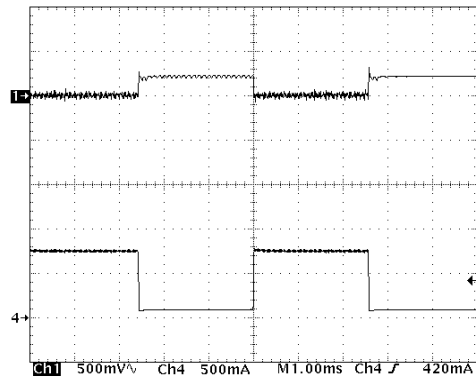
( V_{OUT} = 5.0\text{ V} , I_{LOAD} = 100\text{ mA to }800\text{ mA} ; L = 5.6\text{ }\mu\text{H} , C_{OUT} = 22\text{ }\mu\text{F} ) Upper Trace: Output Voltage Ripple, 500 mV/Division Lower Trace: Load Current, I_{LOAD} , 500 mA/Division
