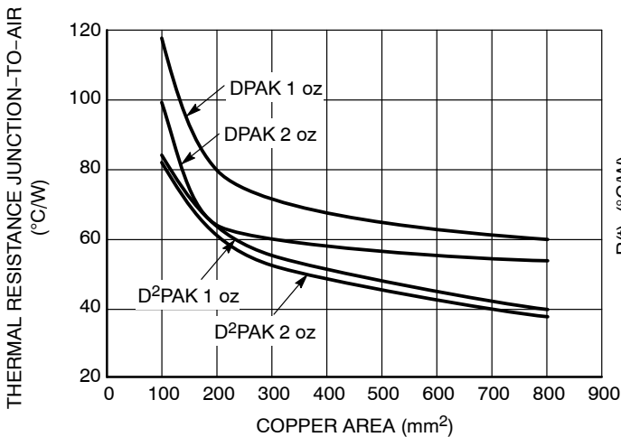
Figure 37. R_{\theta JA} vs. Copper Spreader Area
