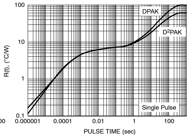
Figure 38. NCV8675 @ PCB Cu Area 100 mm 2 PCB Cu thk 1 oz
