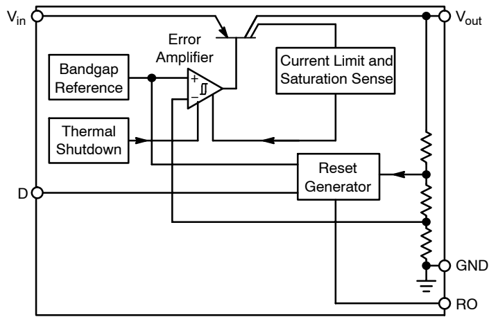
Figure 1. Block Diagram
