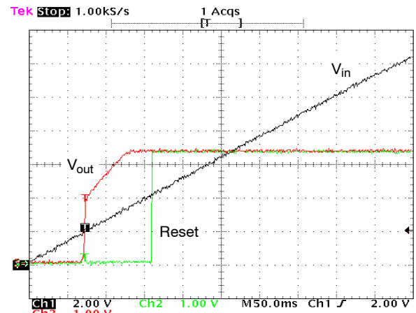
Figure 26. Reset vs. Output Voltage ( V_{in} Rising) (3.3 V Version)
