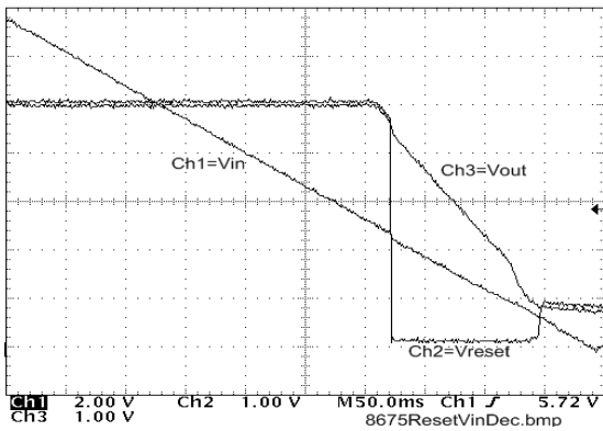
Figure 12. Reset vs. Output Voltage ( V_{in} Falling) (5 V Version)
