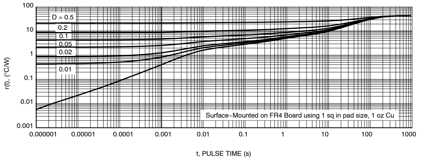
Figure 13. Thermal Response
