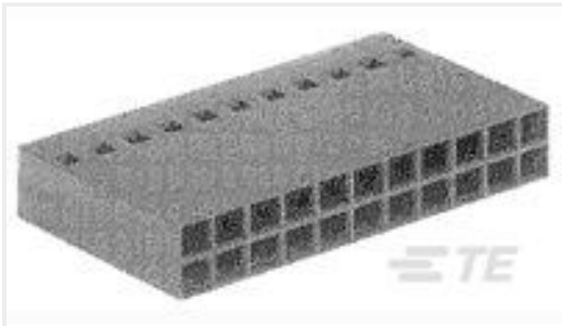
TE Part #1-104482-8 40 SHORT PT RCPT HSG DR .100CL
