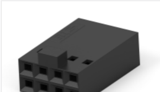
TE Part # 1-103688-0 11 MTE RCPT HSG SR PLAIN .100
