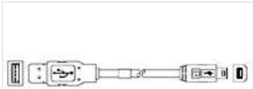
TE Part #1487594-2 USB, A-B, 28/28, BLACK, 0.25M
