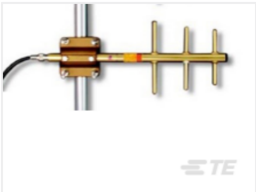
TE Part #Y8963 YAGI,FWG,3,896-970MHz, 6dBi
