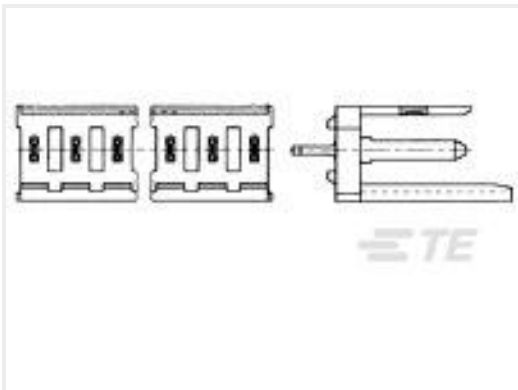
TE Part #280618-1 08P MOD 1 ASSY
