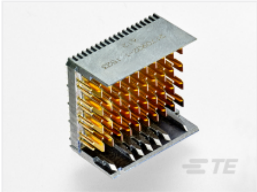
TE Part #2170902-1 HM-EZD+,4PAIRS,10COLS,VERTICAL, ASSEMBLY
