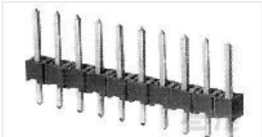
TE Part #3-826926-6 36P AMPMODU II STIFT LEI
