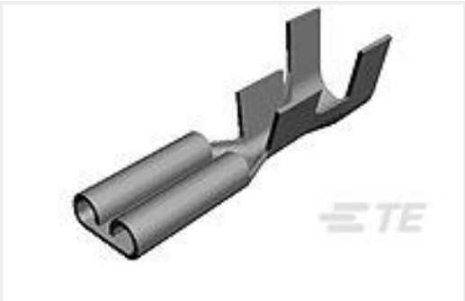
TE Part #5-160431-2 187 FASTON REC 16-14 AWG TPBR
