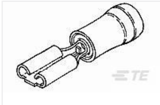
TE Part #8-61060-1 RECEPT,PIDG FASTON 22-18 110
