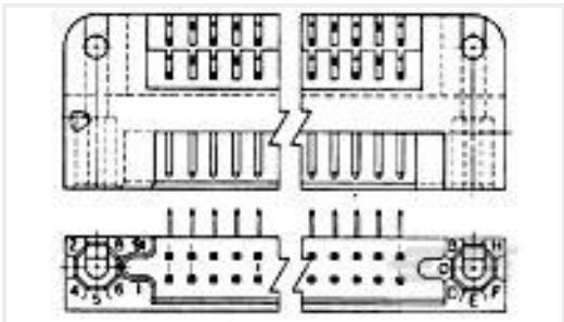
TE Part #531720-9 2 ROW BOX PIN 90 POS R/A
