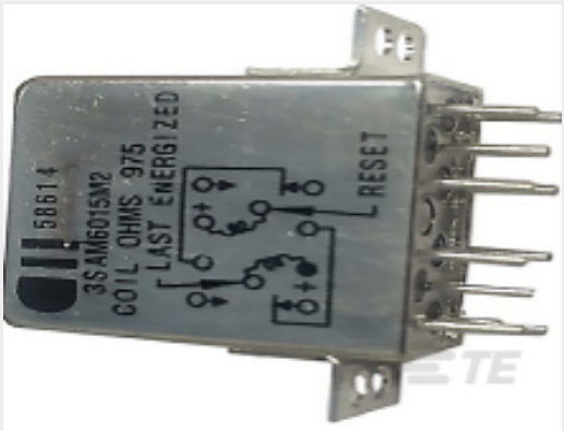
TE Part # 2-1617514-3 3SAT1319A2=M5757/13-102
