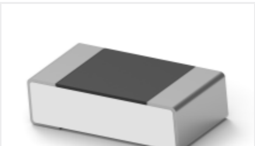
TE Part #3-2176371-5 RQ 0603 10K5 0.1% 10PPM 5K RL
