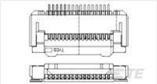
TE Part #3-1734592-0 FPC CONN. 0.5MM PITCH B/C, 30P
