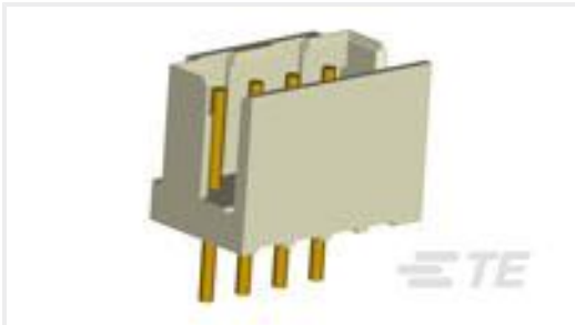
TE Part #292165-4 CT P/HDR BOX V 4P T/P NAT
